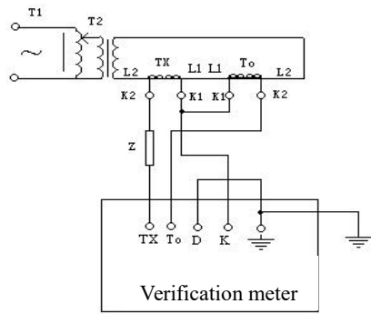
Current transformer error test diagram
