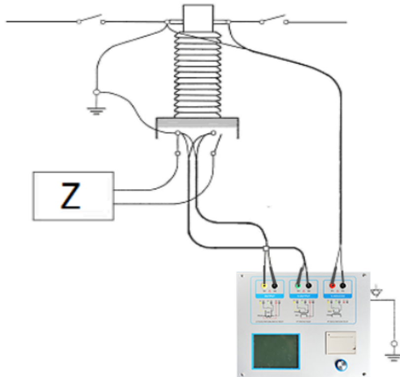
Figure D.1 Typical Connection
