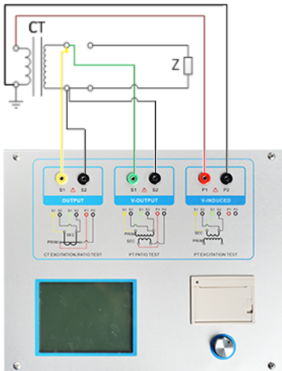
Fig 2.1 DC resistance, excitation, ratio experiment connection
