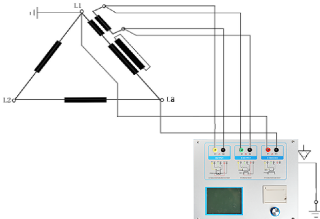
Figure D.2 CTA-1000C in the triangle on the transformer connection when the connection mode test
