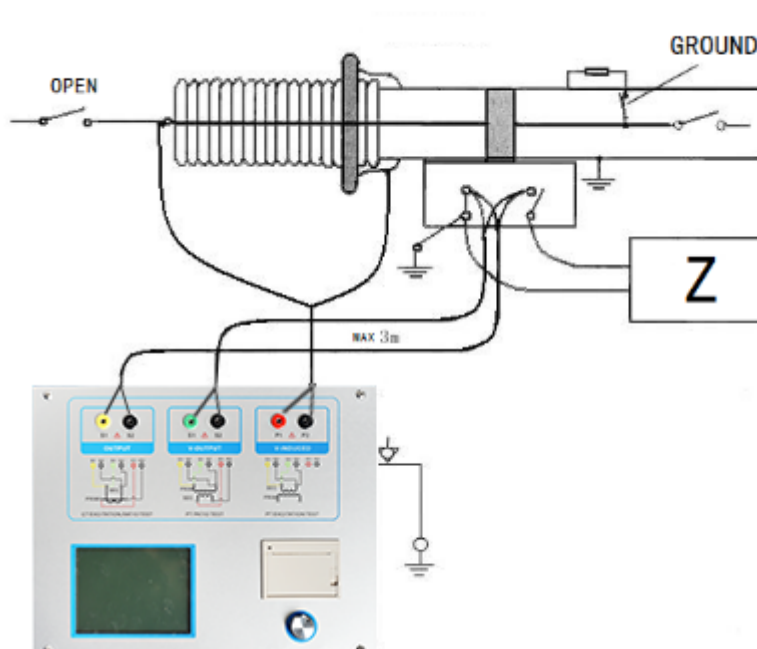
Figure D.4 CTA-1000C on GIS (SF6) switch on the test at the time of CT Connection
