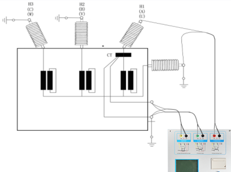
Figure D.3 CTA-1000C on the transformer bushing testing at the time of CT Connection
